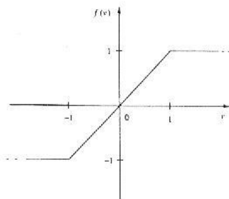
Fig. 4. The characteristic of the nonlinear controlled source.
