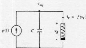
Fig. 6. The steady-state equivalent circuit of a cell in a cellular neural network.
