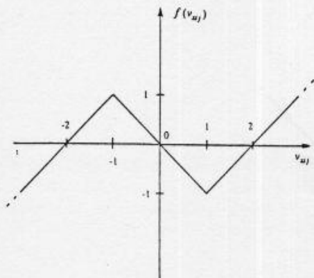
Fig. 5. The characteristic of the nonlinear resistor in the equivalent cell circuit.
