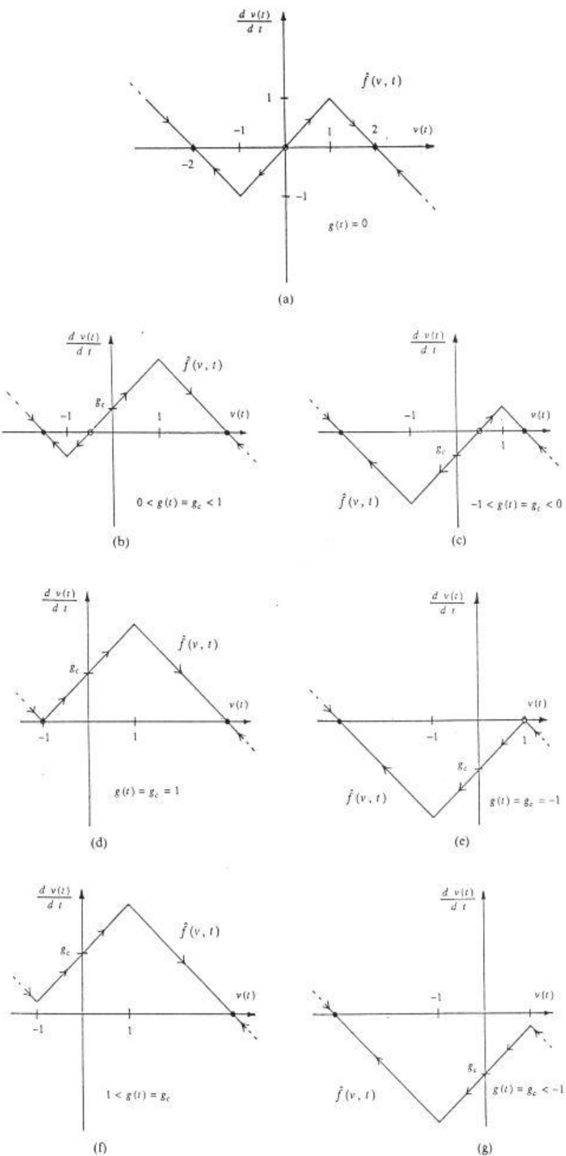
Fig. 7. Dynamic routes and equilibrium points of the equivalent circuit for different values of g(t) .
