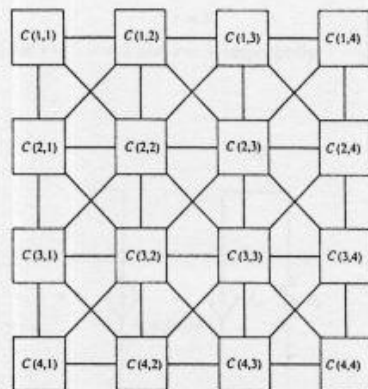
Fig. 1. A two-dimensional cellular neural network. The circuit size is 4 \times 4 . The squares are the circuit units called cells . The links between the cells indicate that there are interactions between the linked cells .
