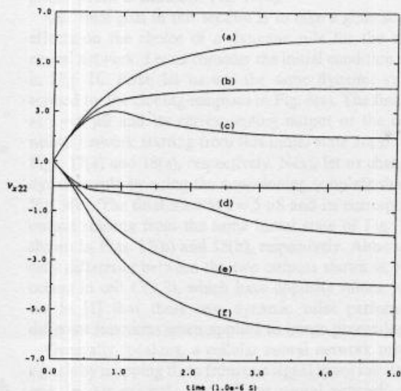
Fig. 12. The transient behaviors of cell C(2,2) corresponding to the initial conditions in Fig. 10.
