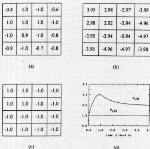
Fig. 9. Computer simulation of a 4 \times 4 cellular neural network. (a) Initial states. (b) Final states. (c) Outputs at steady state. (d) Transient waveforms of cell circuit C(2, 2) .
